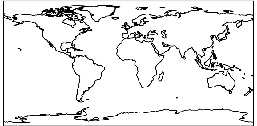
gchp.14.7.0-rc.0 (Dev) c24
