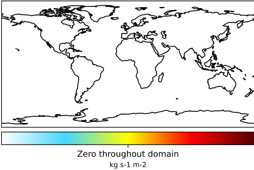
gchp.14.7.0-rc.0 (Dev), Normalized by Area c24
