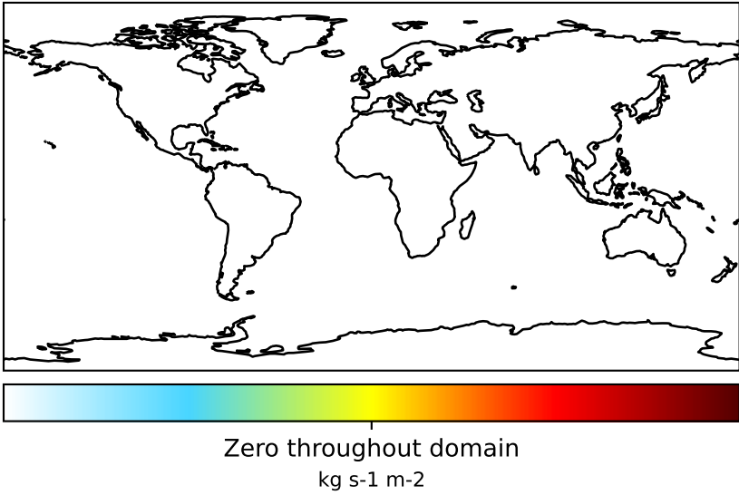
gchp.14.2.0-rc.2 (Ref), Normalized by Area c24
