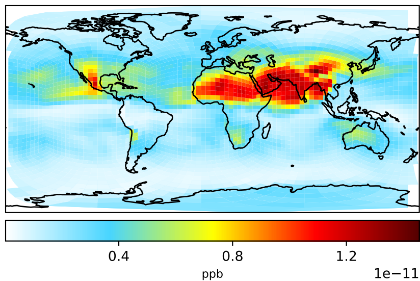
gchp.14.7.0-rc.0 (Ref) c24
