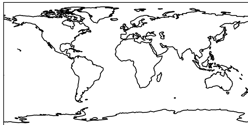
gchp.14.7.0-rc.0-LuoWD (Dev), Normalized by Area c24
